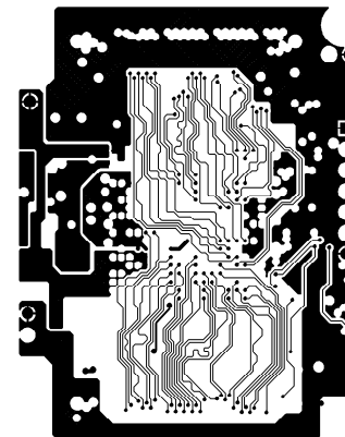
INTERNAL PLANE 4
