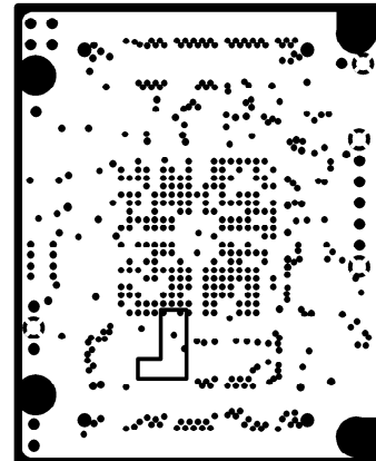
INTERNAL PLANE 2
