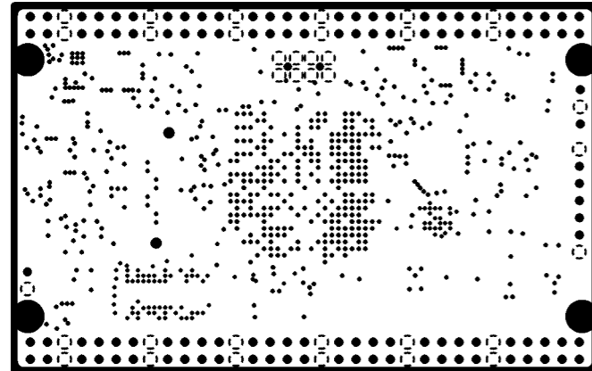
INTERNAL PLANE1(GND)
