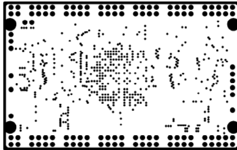
INTERNAL PLANE(GND)
