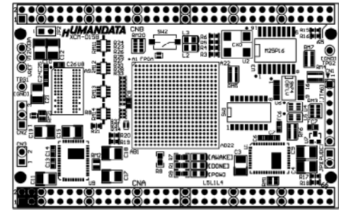
Component Side
