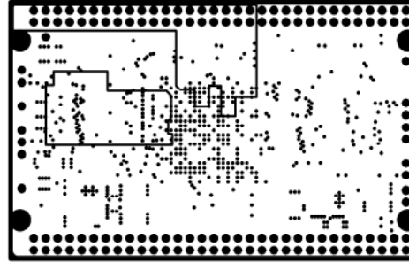
INTERNAL PLANE2
