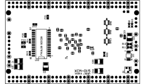
Solder Side
