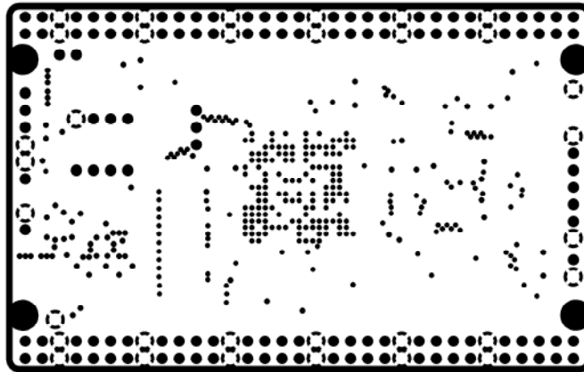
INTERNAL PLANE(GND)
