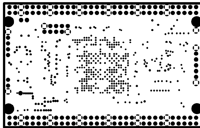
INTERNAL PLANE1(GND)
