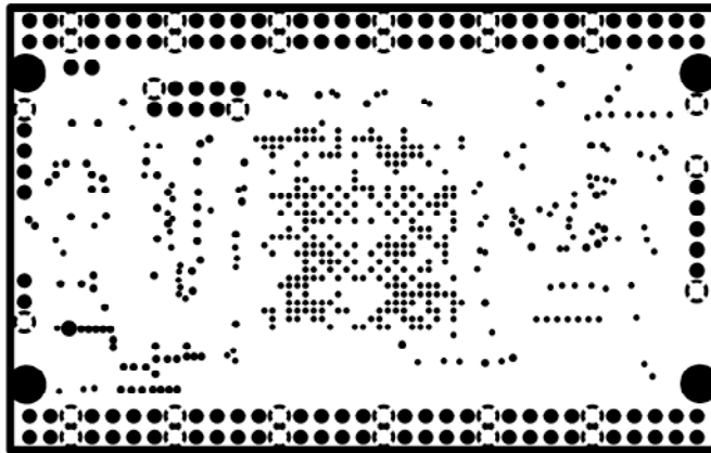
INTERNAL PLANE1(GND)
