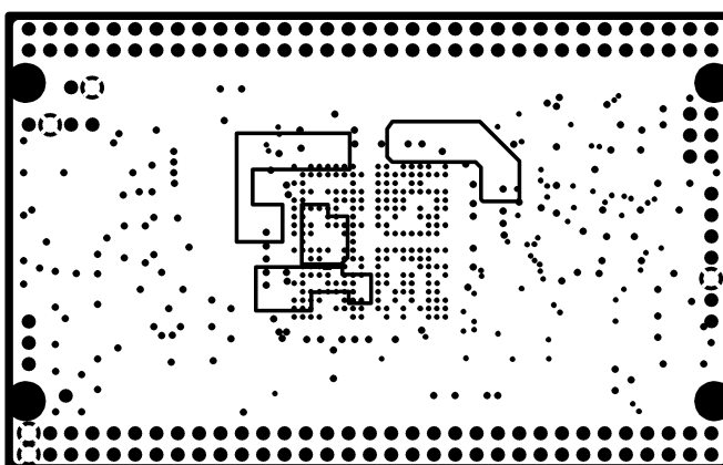
INTERNAL PLANE2
