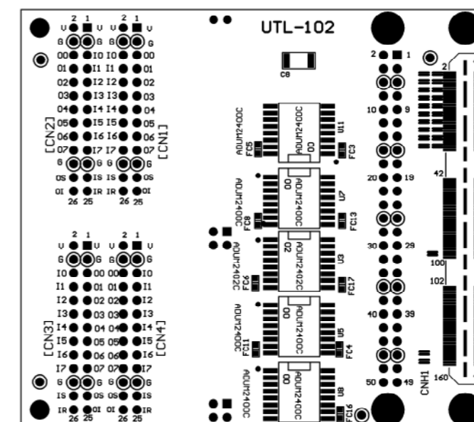
Solder Side
