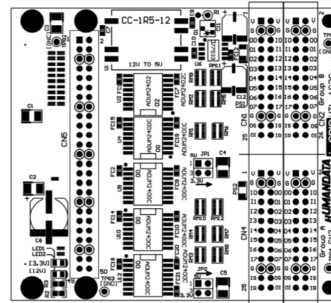
Component Side
