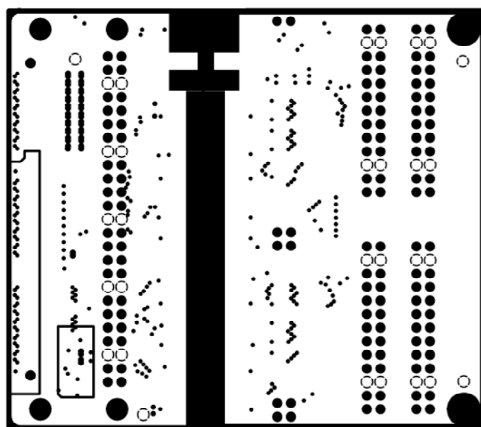
INTERNAL PLANE1
