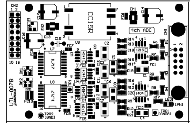
Component Side
