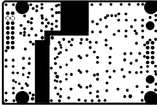
INTERNAL PLANE2
