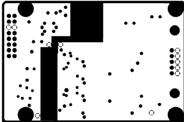
INTERNAL PLANE1
