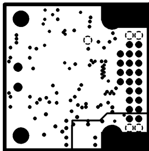
INTERNAL PLANE1
