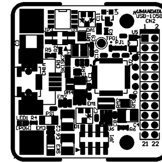
Component Side
