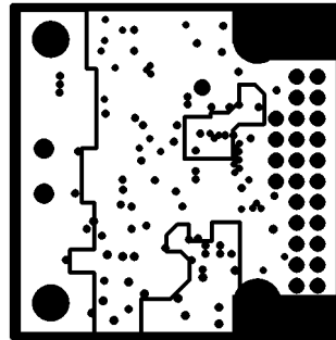
INTERNAL PLANE2
