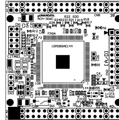
Component Side
