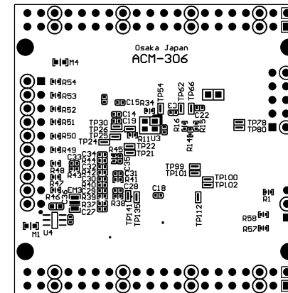
Solder Side
