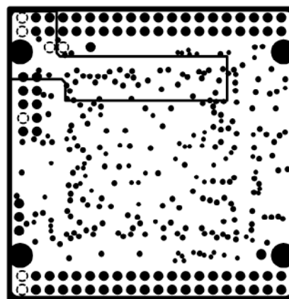
INTERNAL PLANE4
