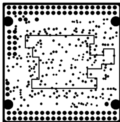
INTERNAL PLANE3
