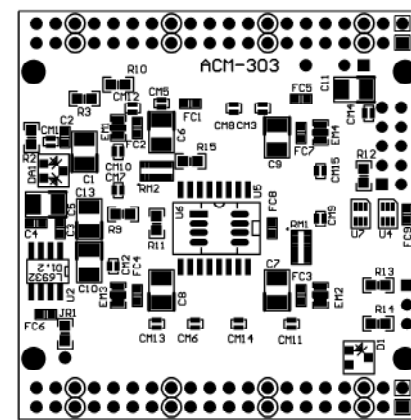
Solder Side
