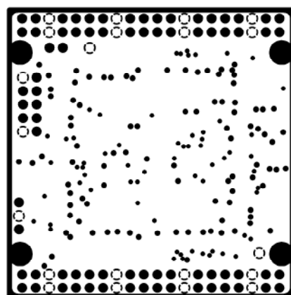
INTERNAL PLANE1
