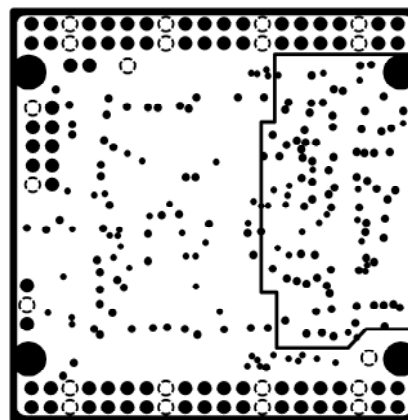
INTERNAL PLANE2
