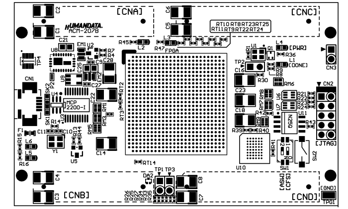
Component Side
