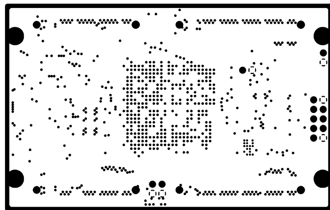
INTERNAL PLANE 1
