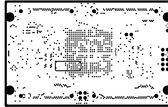
INTERNAL PLANE 2
