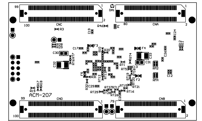
Solder Side
