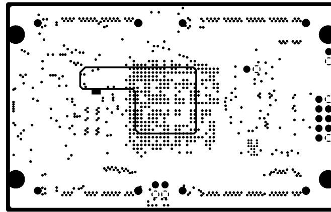
INTERNAL PLANE 4
