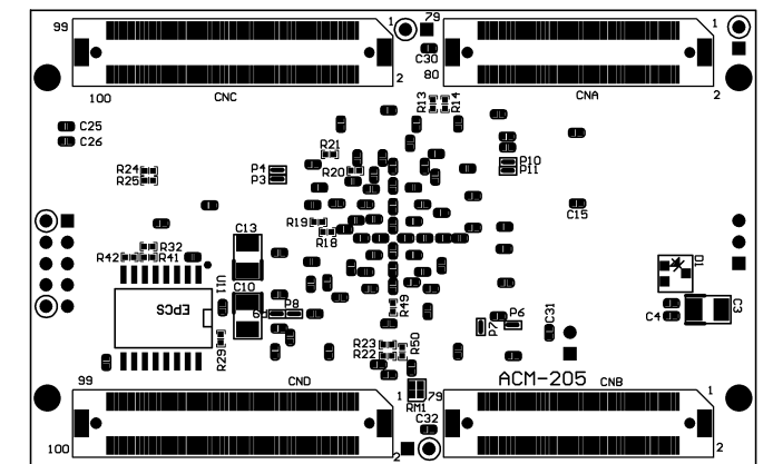
Solder Side
