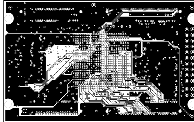
MidLayer5 (Scale 1:1)
