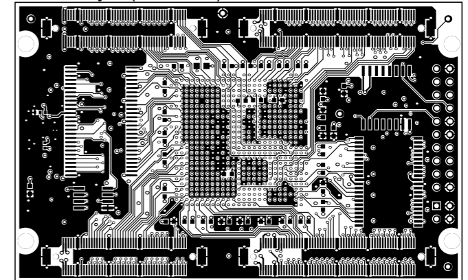
BottomLayer (Scale 1:1)
