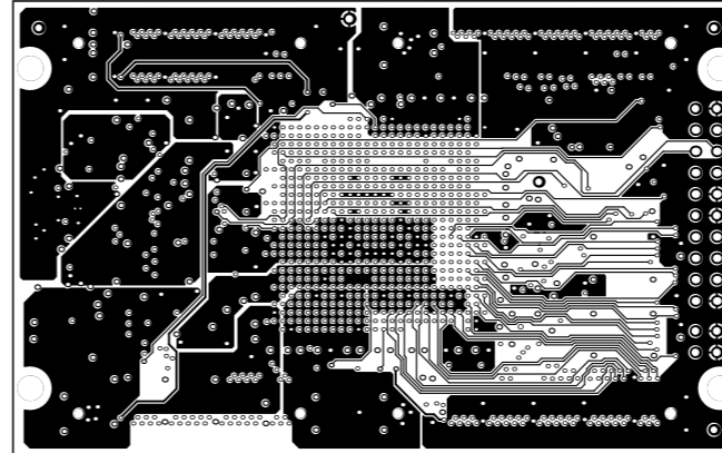
MidLayer6 (Scale 1:1)
