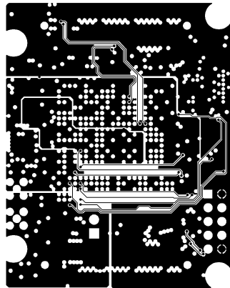
MID LAYER4
