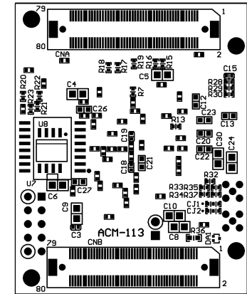
Solder Side
