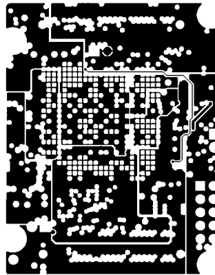
MID LAYER4
