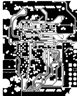
MID LAYER3
