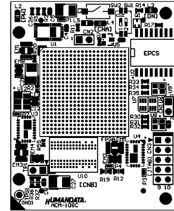
Component Side
