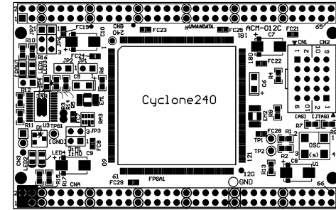
Component Side
