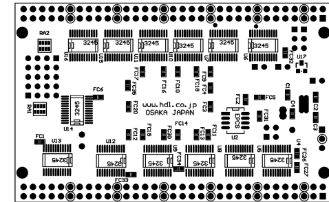
Solder Side
