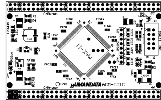
Component Side
