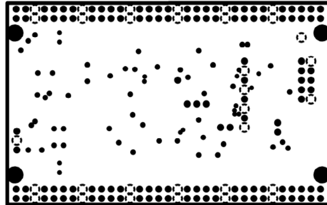
INTERNAL PLANE1(GND)
