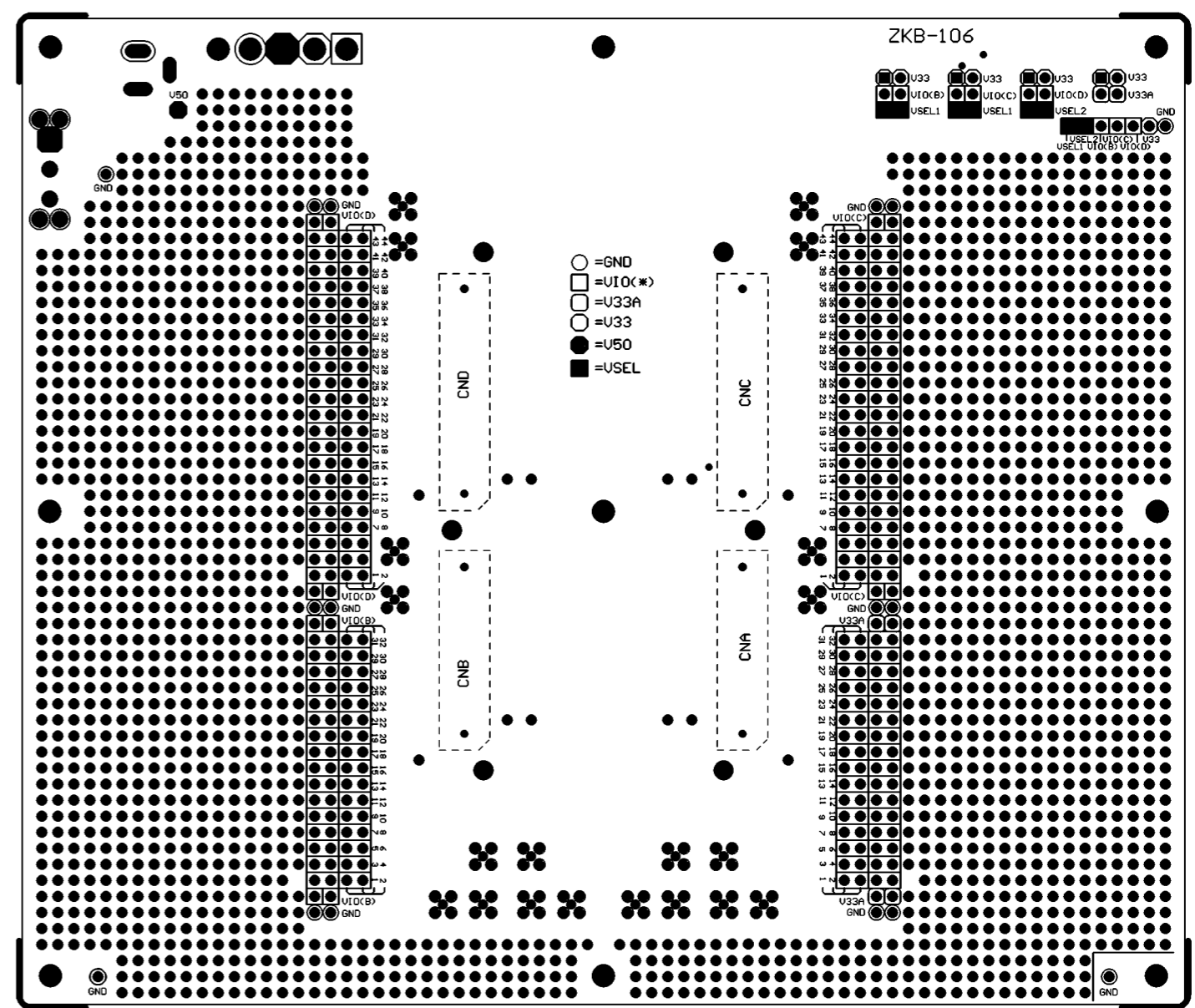
Solder Side
