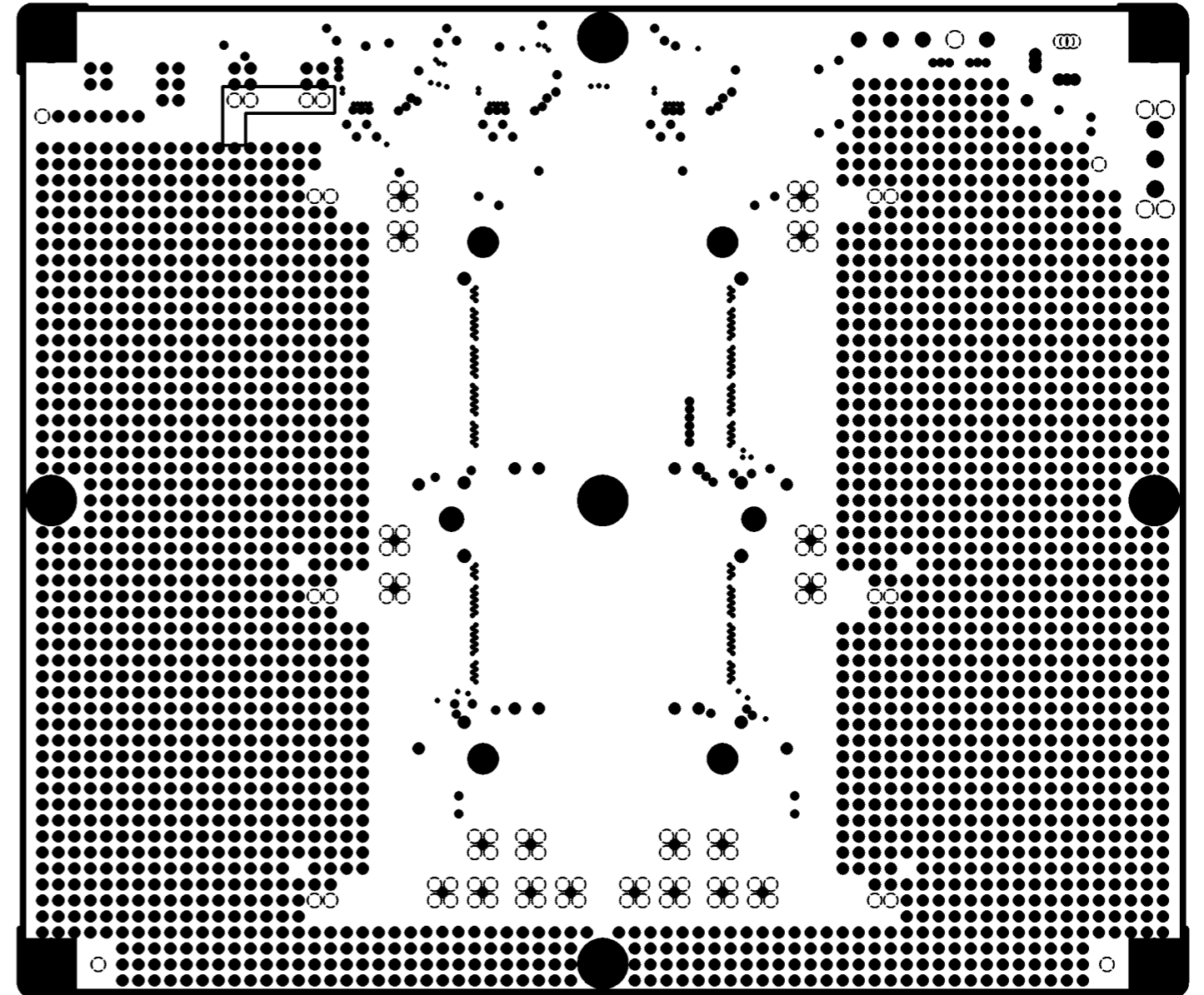
INTERNAL PLANE1
