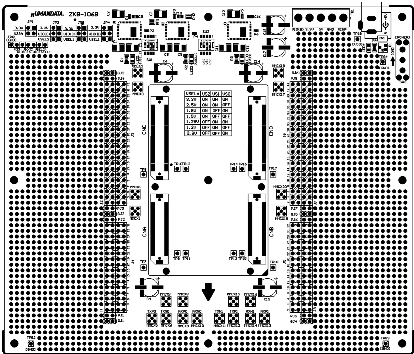
Component Side
