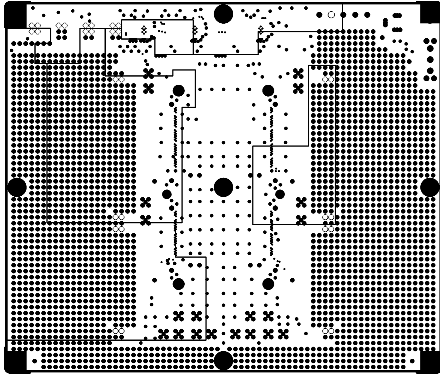
INTERNAL PLANE2
