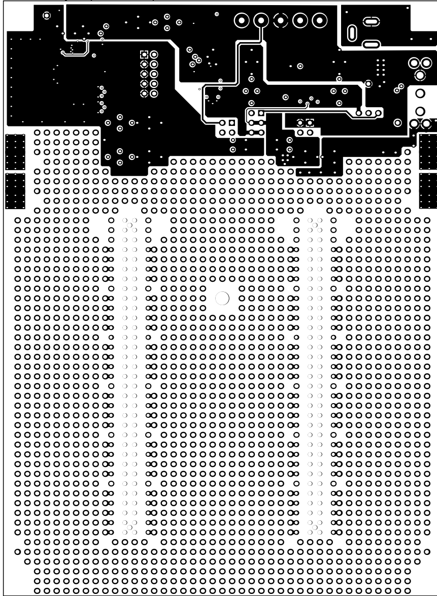
BottomLayer (Scale 1:1)
