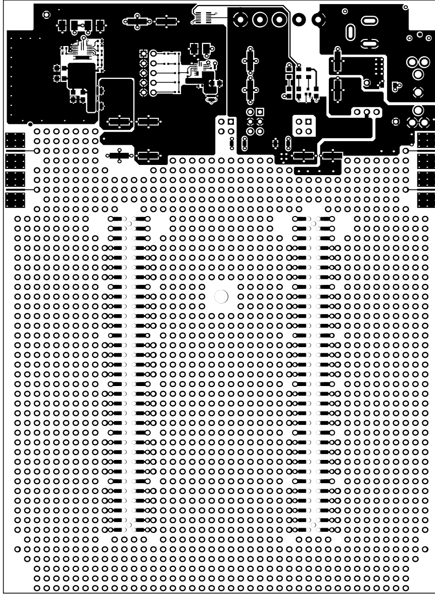
TopLayer (Scale 1:1)
