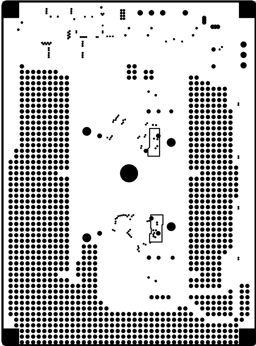
INTERNAL PLANE1
