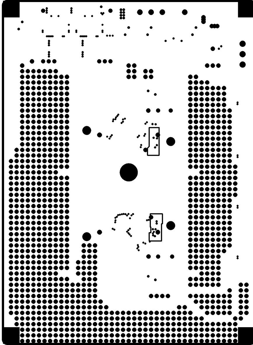
INTERNAL PLANE1
