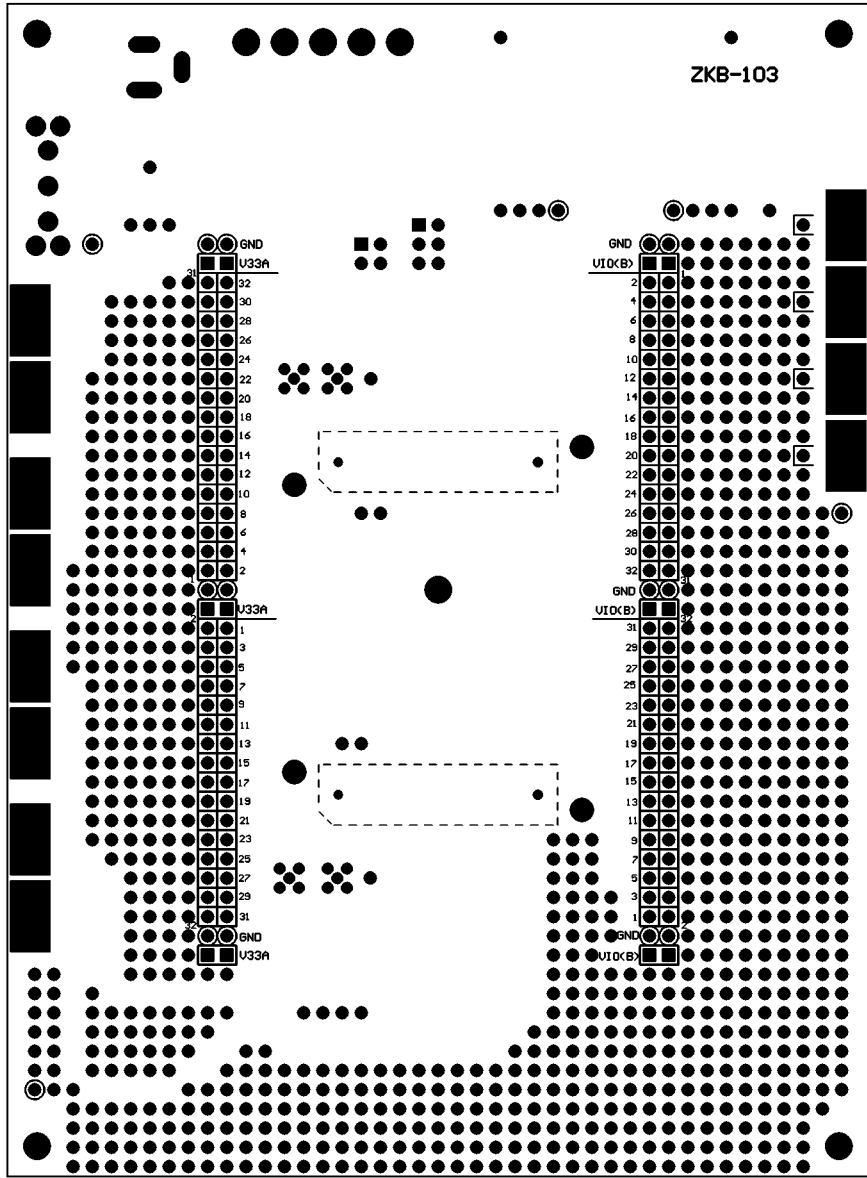
Solder Side
