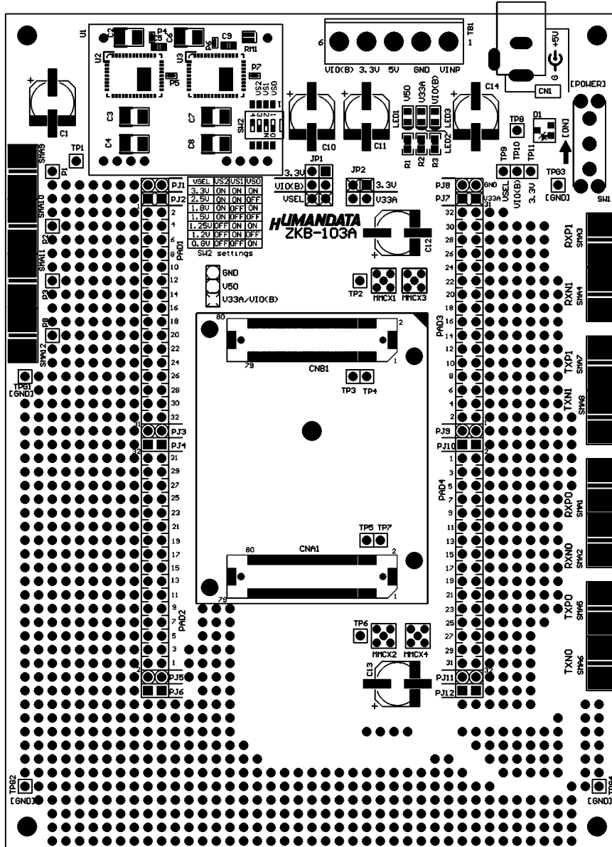
Component Side
