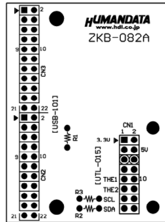
Component Side
