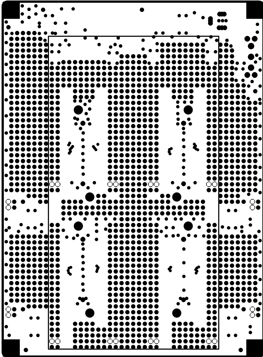
INTERNAL PLANE2
