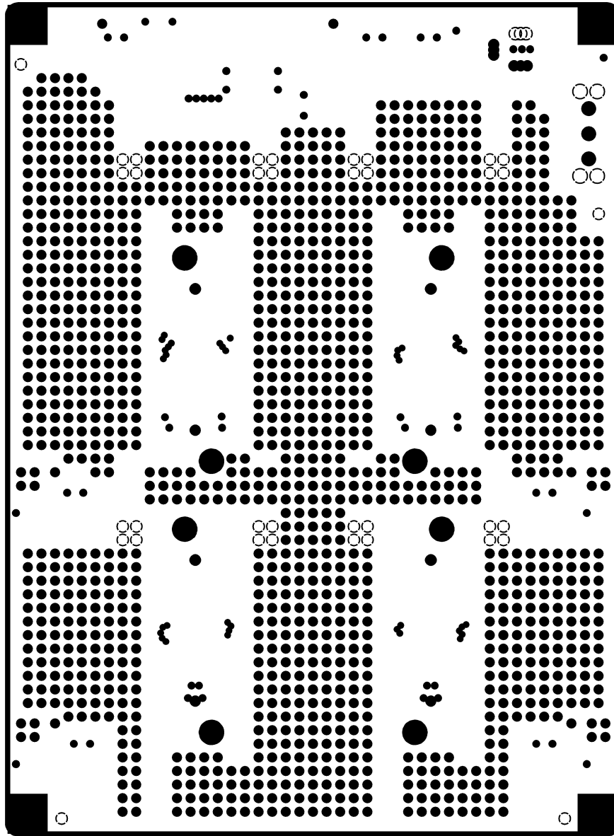
INTERNAL PLANE1
