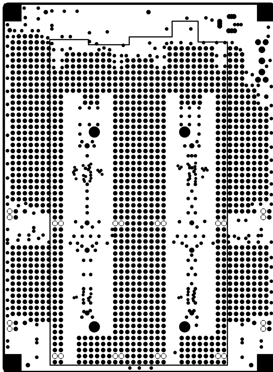
INTERNAL PLANE2
