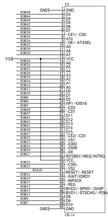
CF CARD
