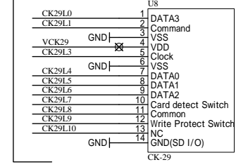
SD CARD
