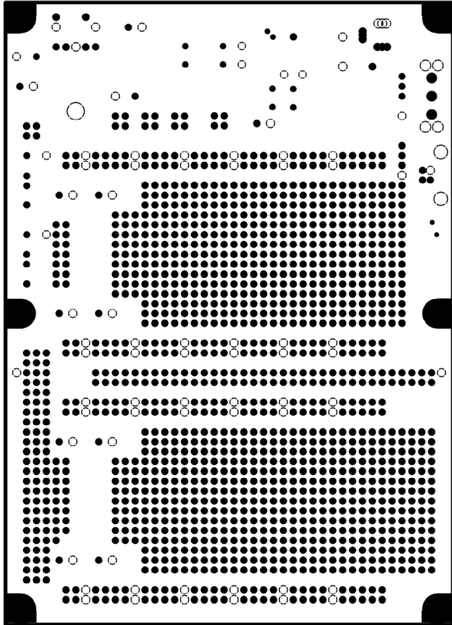
INTERNAL PLANE1
