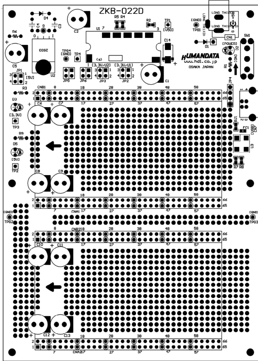
Component Side
