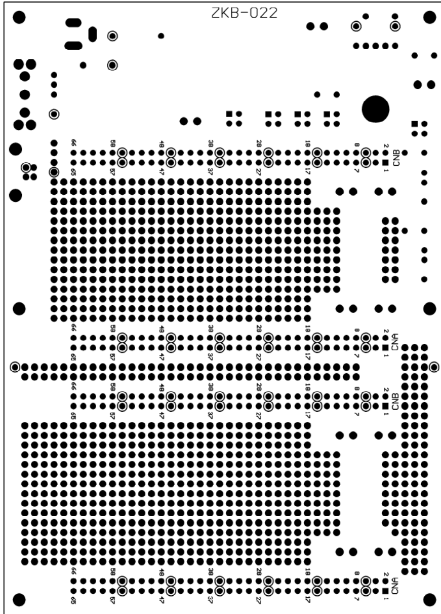
Solder Side
