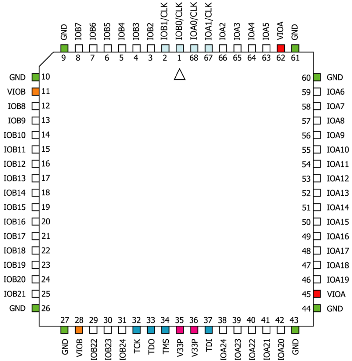
TOP VIEW
