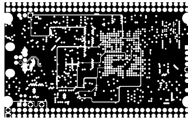
MID LAYER4
