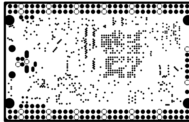
INTERNAL PLANE(VCC)
