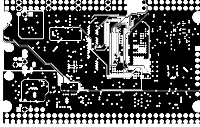
MID LAYER3
