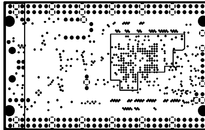
INTERNAL PLANE2
