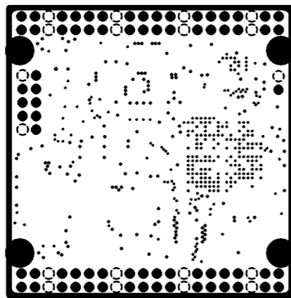
INTERNAL PLANE1
