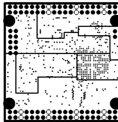
INTERNAL PLANE4
