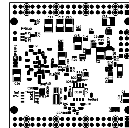
Solder Side
