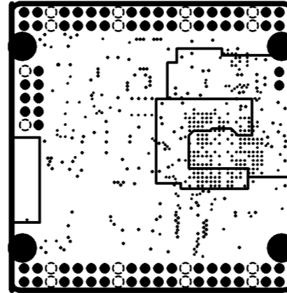
INTERNAL PLANE3
