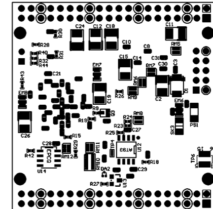
Solder Side
