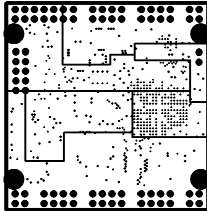
INTERNAL PLANE4
