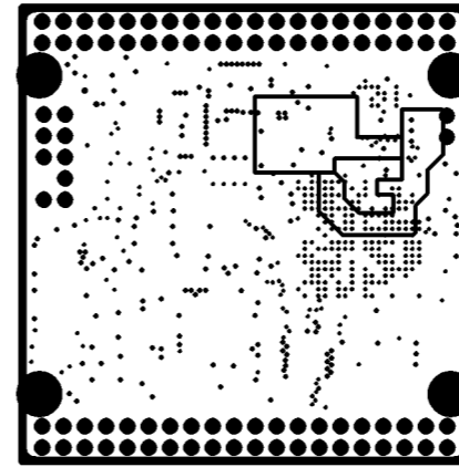
INTERNAL PLANE2
