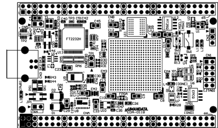
Component Side
