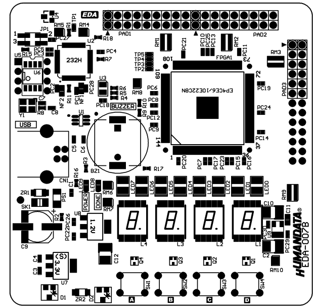
Component Side
