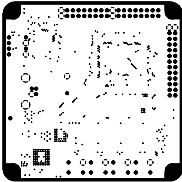
INTERNAL PLANE1
