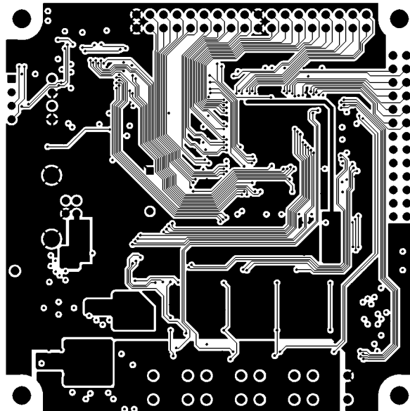
INTERNAL PLANE2
