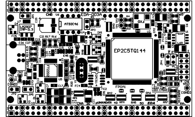
Component Side
