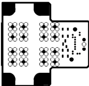
INTERNAL PLANE1
