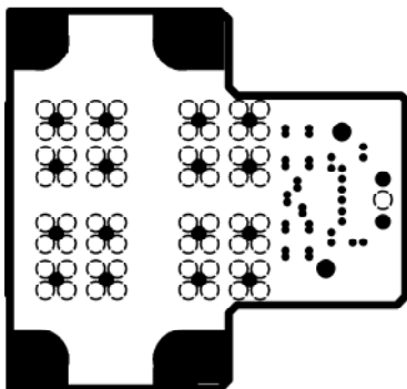
INTERNAL PLANE2
