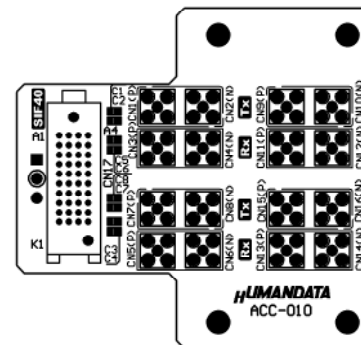
Solder Side
