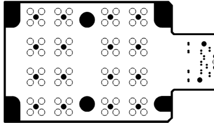
INTERNAL PLANE2
