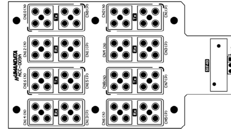
Component Side
