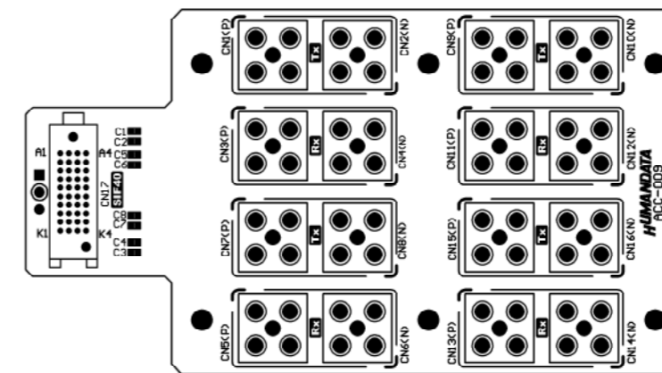
Solder Side
