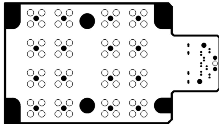
INTERNAL PLANE1
