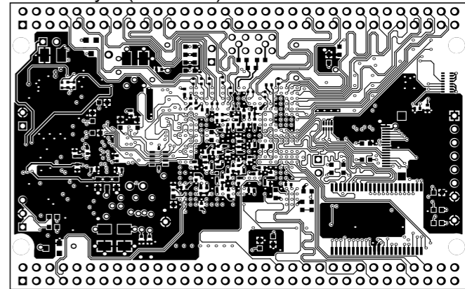
BottomLayer (Scale 1:1)
