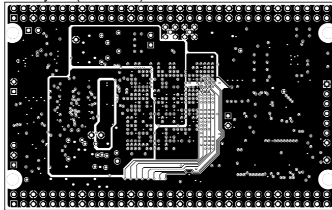
MidLayer3 (Scale 1:1)
