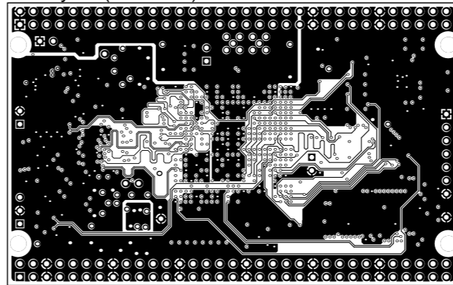
MidLayer2 (Scale 1:1)
