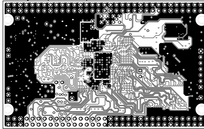
MidLayer1 (Scale 1:1)
