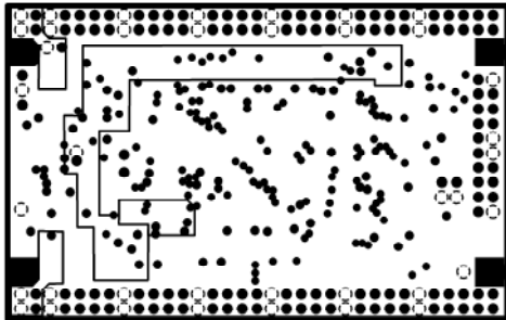
INTERNAL PLANE1
