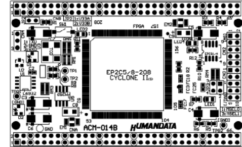
Component Side
