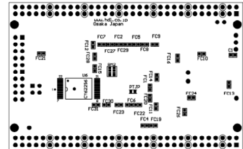
Solder Side
