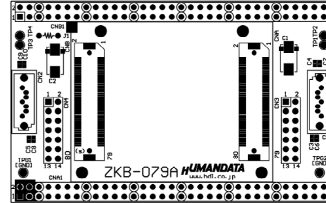
Component Side
