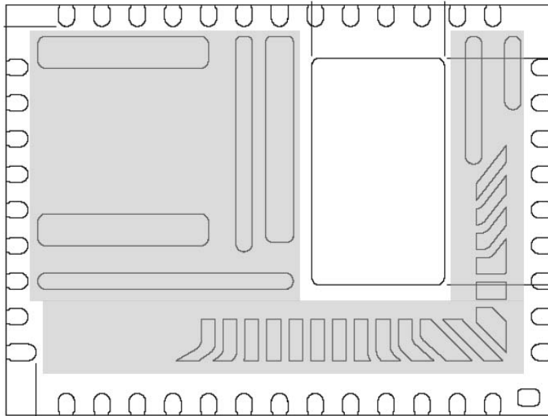
Figure 4. Lead-Frame exposed metal. Grey area highlights exposed metal that is not to be mechanically or electrically connected to the PWB.
