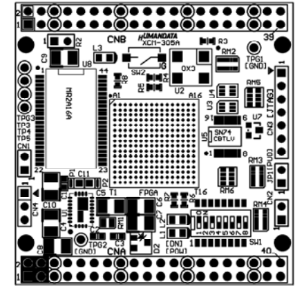
Component Side
