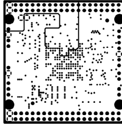
INTERNAL PLANE2
