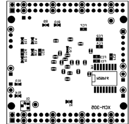
Solder Side
