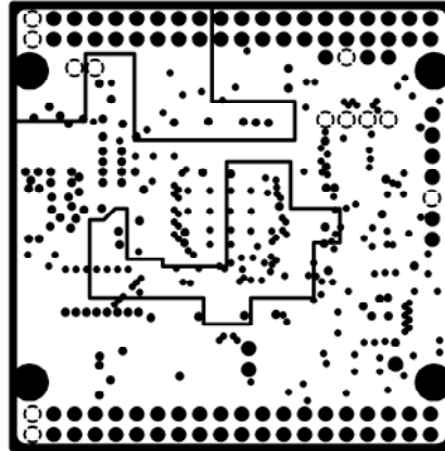
INTERNAL PLANE2(VCC)
