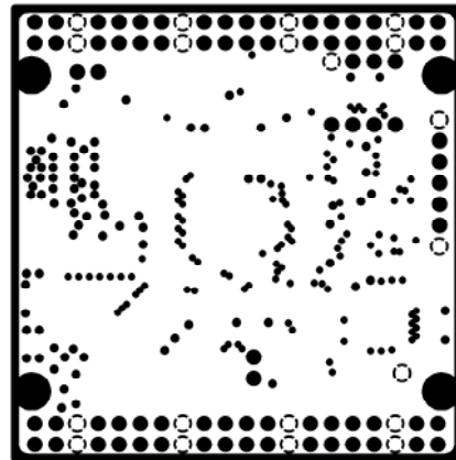
INTERNAL PLANE1(GND)
