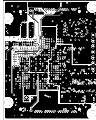
MidLayer4 (Scale 1:1)
