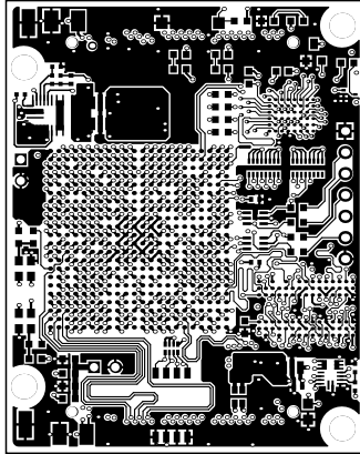
TopLayer (Scale 1:1)
