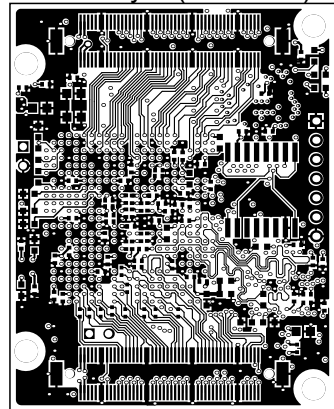
BottomLayer (Scale 1:1)
