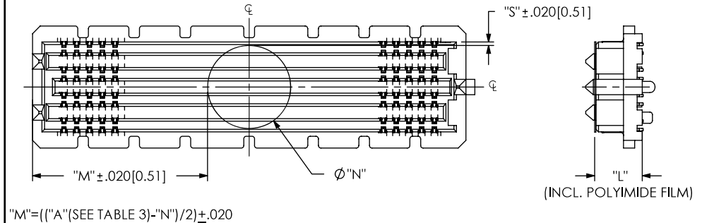
FIG. 4 -K: POLYIMIDE PAD (SEAM-30-02.0-XX-08-1-A-XX-K-TR SHOWN) (SAME AS FIG. 1, EXCEPT AS SHOWN) (ALL CONTACTS NOT SHOWN FOR CLARITY)
