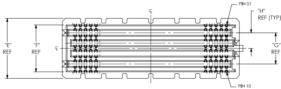
FIG. 2 -10: 10 ROW (SAME AS FIG. 1, EXCEPT AS SHOWN) (SEAM-30-02.0-XX-10-1-A-XX-K-TR SHOWN) (SOME CENTER FEATURES, INCLUDING -K, NOT SHOWN FOR CLARITY)
