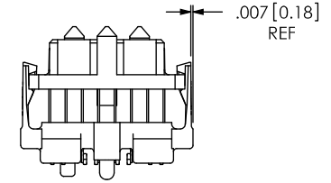
-07.0 LEAD STYLE (SEAM-XX-07.0-X-08-A-X SHOWN)
