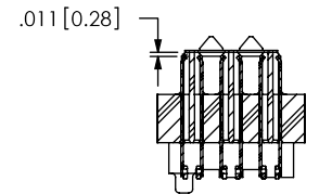
SECTION "G"-"G"
