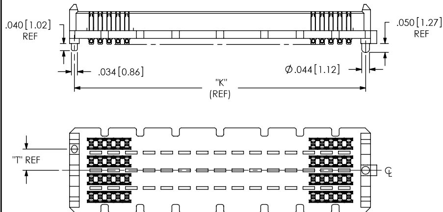
FIG. 3 -A: ALIGNMENT PINS APPLIES TO ALL -A OPTION PART NUMBERS (SAME AS FIG. 1, EXCEPT AS SHOWN) (SEAM-30-02.0-XX-08-1-A-XX-K-TR SHOWN) (SOME CONTACTS NOT SHOWN FOR CLARITY)
