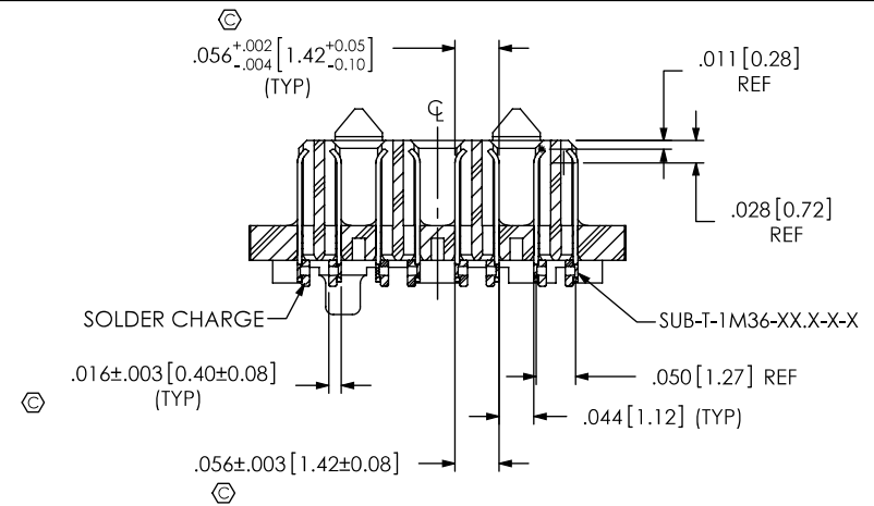
FIG. 4 -K: POLYIMIDE PAD (SEAM-30-02.0-XX-08-1-A-XX-K-TR SHOWN) (SAME AS FIG. 1, EXCEPT AS SHOWN) (ALL CONTACTS NOT SHOWN FOR CLARITY)
